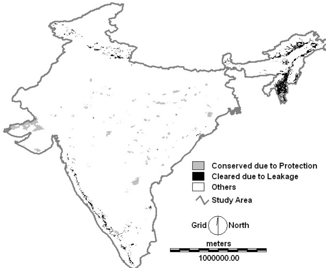
Figure 4. Map of displacement where where baseline clearing inside protected areas is displaced to locations outside protected areas.
