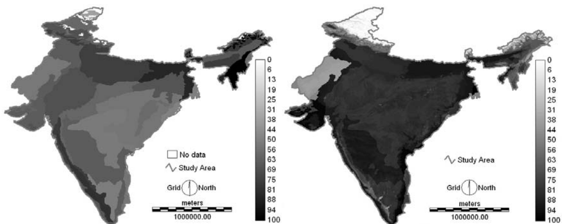
Figure 2. (a) Suitability for conservaiton on the left, and (b) suitability for development on the right.
