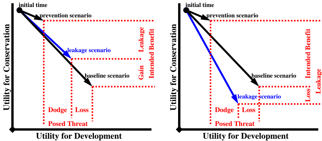
Figure 5. (a) Theoretical intended arrangement of points on the left, and (b) observed arrangement of points for the Indian case study on the right.
