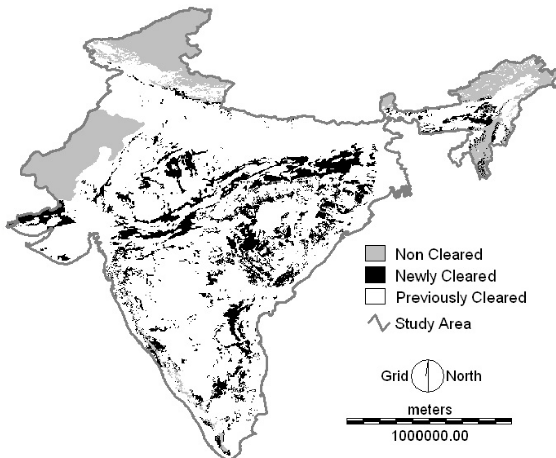
Figure 3. Baseline scenario of future where newly cleared areas occur in places of high suitability for development, regardless of protected status.
