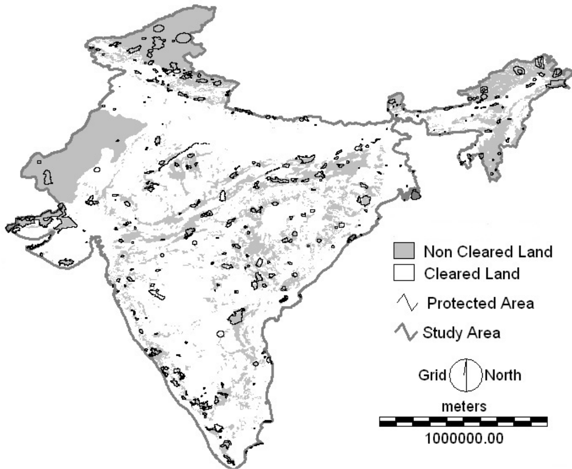
Figure 1. Initial cleared areas and protected areas.
