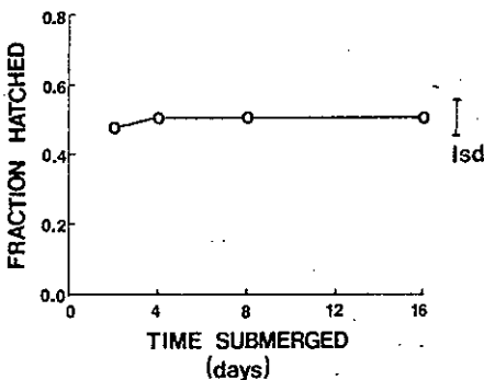
FIG. 1. Fraction of Aedes triseriatus eggs hatching as a function of time submerged in natural treeholes. Mean hatch rates are shown, pooled across all levels of larval density. Hatch rate is shown in units of radians, which resulted from the use of the transformation y' = a \sin \sqrt{y} , where y is the fraction of eggs hatched per batch. Tukey's least significant difference (lsd) is shown for visual comparison of means.
