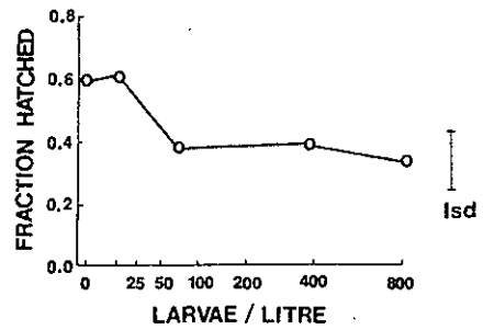
FIG. 2. Fraction of Aedes triseriatus eggs hatching in response to density of larvae in natural treeholes. Density is plotted on a square root scale. Mean hatching fractions are shown, pooled across all time intervals. Hatch rate is shown in units of radians, which resulted from the transformation y' = a \sin \sqrt{y} , where y is the fraction of eggs hatched per batch. Tukey's least significant difference (lsd) is shown for visual comparison of means.
