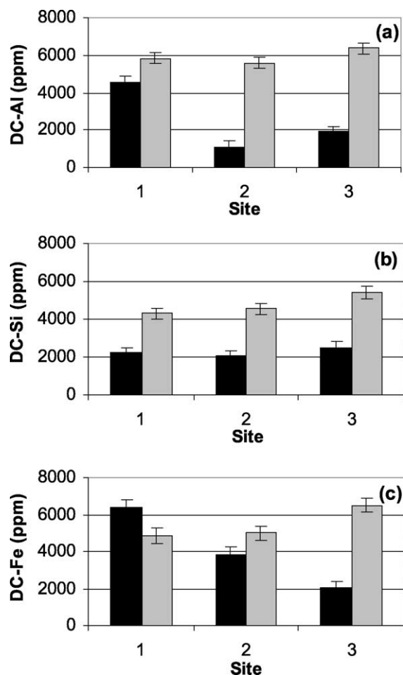
Fig. 5. Selective dissolution results from B-horizon soil collected in September 1999. Dithionite-citrate extractable (a) Al (DC-Al), (b) Si (DC-Si), (c) Fe (DC-Fe). Error bars represent range of duplicate samples. Black = high-CO 2 soil. Grey = control soil.
